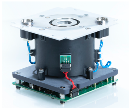
Figure 2 IFM Nano Thruster
