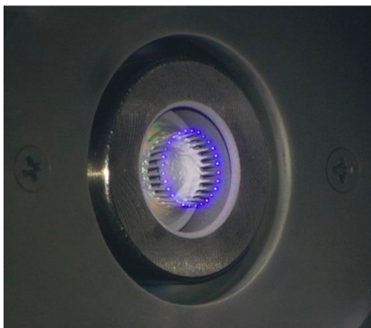
Figure 1 Closeup of IFM emitter during ion emission
